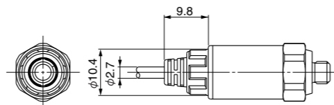
With sensor cable fitted
